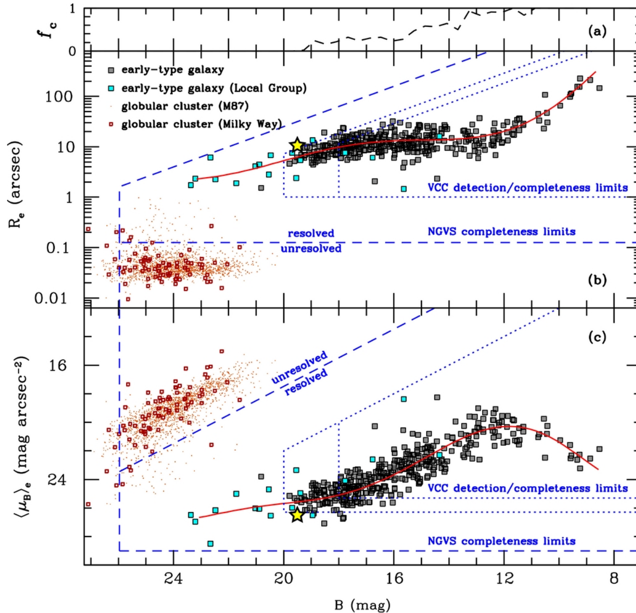
Figure 16. from The Next Generation Virgo Cluster Survey (NGVS). I. Introduction to the Survey Ferrarese et al. 2012 ApJS 200 4 doi:10.1088/0067-0049/200/1/4 https://dx.doi.org/10.1088/0067-0049/200/1/4 © 2012. The American Astronomical Society. All rights reserved.
