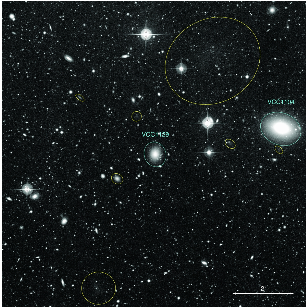
Figure 15. from The Next Generation Virgo Cluster Survey (NGVS). I. Introduction to the Survey Ferrarese et al. 2012 ApJS 200 4 doi:10.1088/0067-0049/200/1/4 https://dx.doi.org/10.1088/0067-0049/200/1/4 © 2012. The American Astronomical Society. All rights reserved.
