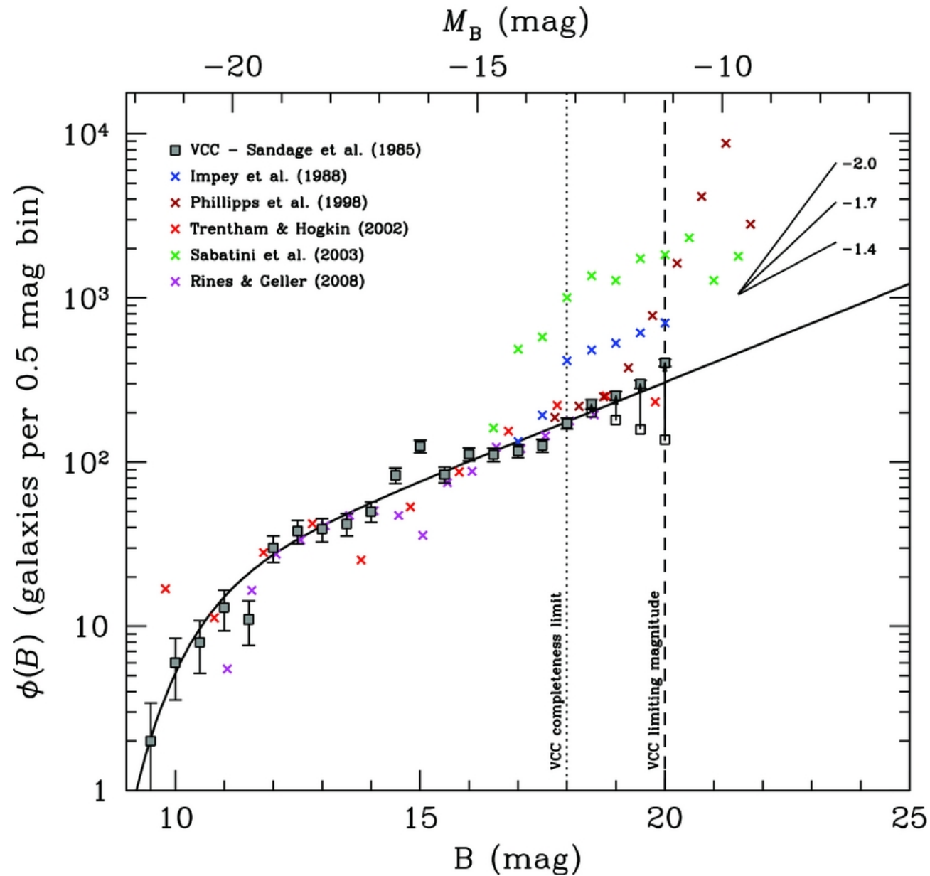
Figure 14. from The Next Generation Virgo Cluster Survey (NGVS). I. Introduction to the Survey Ferrarese et al. 2012 ApJS 200 4 doi:10.1088/0067-0049/200/1/4 https://dx.doi.org/10.1088/0067-0049/200/1/4 © 2012. The American Astronomical Society. All rights reserved.
