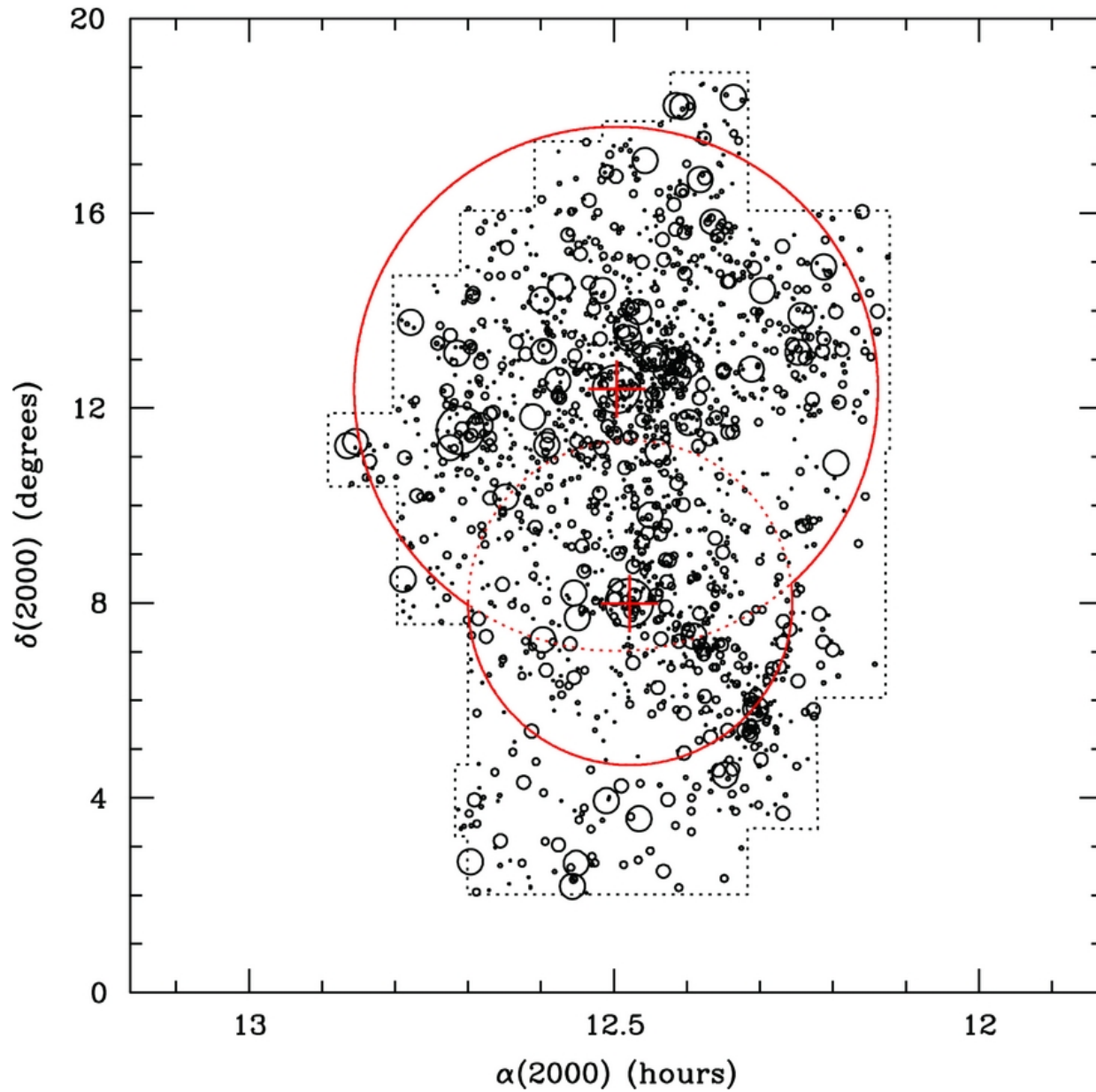
Figure 1. from The Next Generation Virgo Cluster Survey (NGVS). I. Introduction to the Survey Ferrarese et al. 2012 ApJS 200 4 doi:10.1088/0067-0049/200/1/4 https://dx.doi.org/10.1088/0067-0049/200/1/4 © 2012. The American Astronomical Society. All rights reserved.
