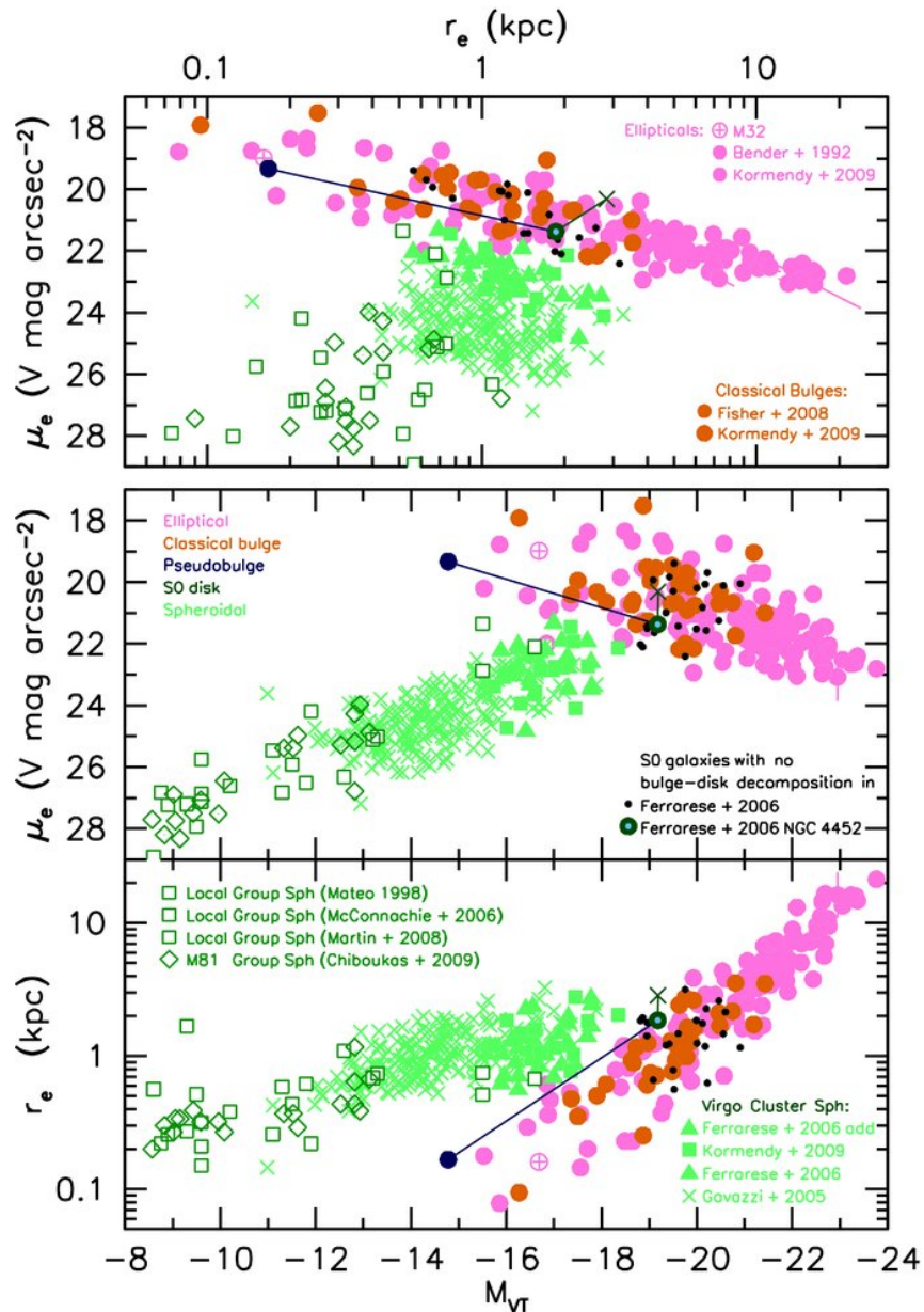
Figure 9. from A Revised Parallel-sequence Morphological Classification of Galaxies: Structure and Formation of S0 and Spheroidal Galaxies Kormendy & Bender 2012 ApJS 198 2 doi:10.1088/0067-0049/198/1/2 https://dx.doi.org/10.1088/0067-0049/198/1/2 © 2012. The American Astronomical Society. All rights reserved.
