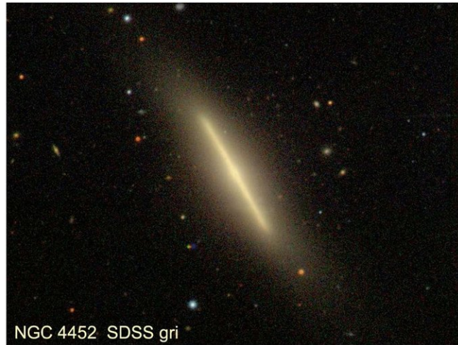
Figure 8. from A Revised Parallel-sequence Morphological Classification of Galaxies: Structure and Formation of S0 and Spheroidal Galaxies Kormendy & Bender 2012 ApJS 198 2 doi:10.1088/0067-0049/198/1/2 https://dx.doi.org/10.1088/0067-0049/198/1/2 © 2012. The American Astronomical Society. All rights reserved.
