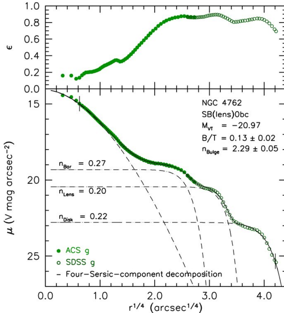
Figure 6. from A Revised Parallel-sequence Morphological Classification of Galaxies: Structure and Formation of S0 and Spheroidal Galaxies Kormendy & Bender 2012 ApJS 198 2 doi:10.1088/0067-0049/198/1/2 https://dx.doi.org/10.1088/0067-0049/198/1/2 © 2012. The American Astronomical Society. All rights reserved.
