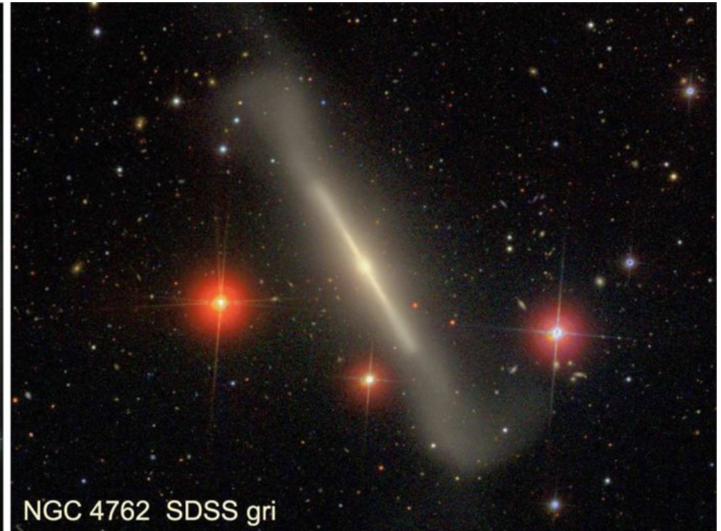
Figure 4. from A Revised Parallel-sequence Morphological Classification of Galaxies: Structure and Formation of S0 and Spheroidal Galaxies Kormendy & Bender 2012 ApJS 198 2 doi:10.1088/0067-0049/198/1/2 https://dx.doi.org/10.1088/0067-0049/198/1/2 © 2012. The American Astronomical Society. All rights reserved.
