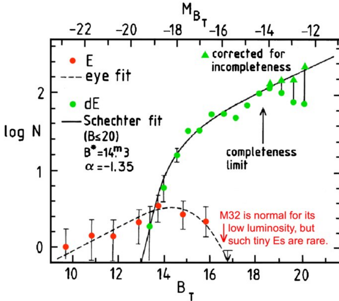
Figure 3. from A Revised Parallel-sequence Morphological Classification of Galaxies: Structure and Formation of S0 and Spheroidal Galaxies Kormendy & Bender 2012 ApJS 198 2 doi:10.1088/0067-0049/198/1/2 https://dx.doi.org/10.1088/0067-0049/198/1/2 © 2012. The American Astronomical Society. All rights reserved.
