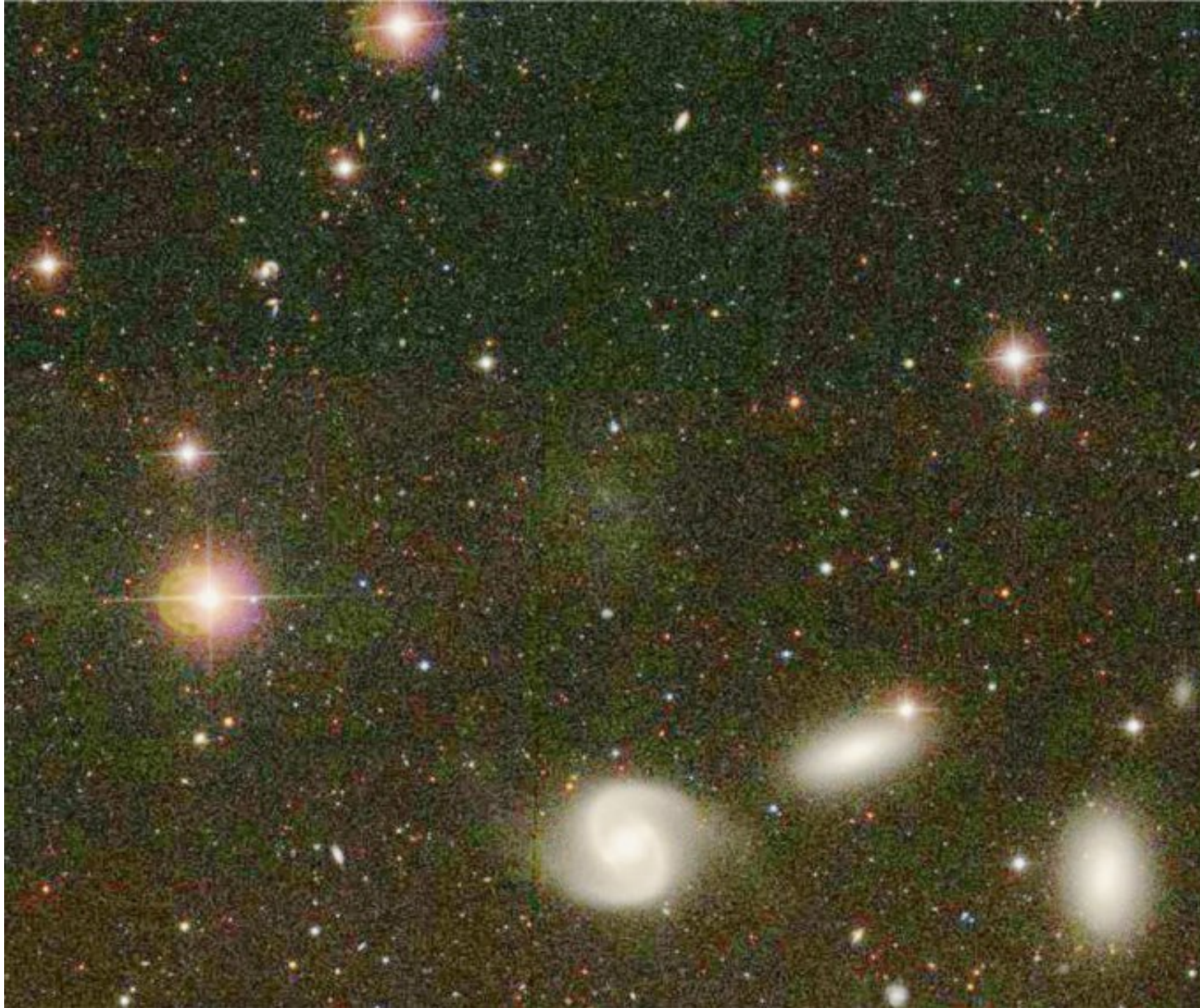
Figure 27. from A Revised Parallel-sequence Morphological Classification of Galaxies: Structure and Formation of S0 and Spheroidal Galaxies Kormendy & Bender 2012 ApJS 198 2 doi:10.1088/0067-0049/198/1/2 https://dx.doi.org/10.1088/0067-0049/198/1/2 © 2012. The American Astronomical Society. All rights reserved.
