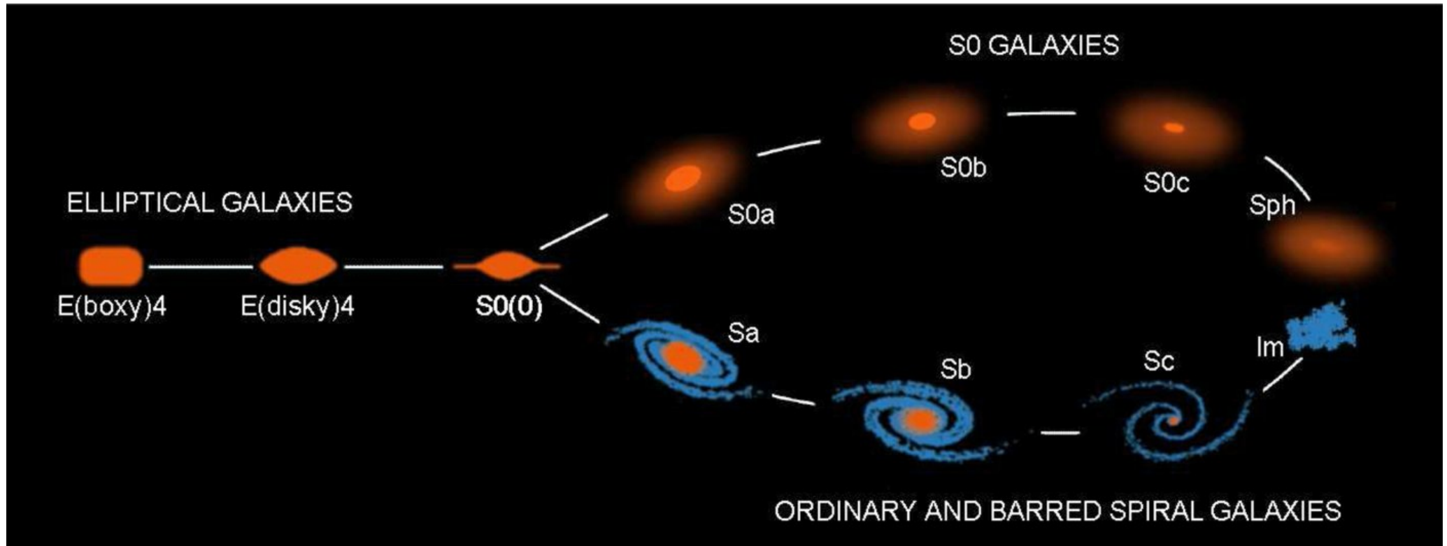
Figure 1. from A Revised Parallel-sequence Morphological Classification of Galaxies: Structure and Formation of S0 and Spheroidal Galaxies Kormendy & Bender 2012 ApJS 198 2 doi:10.1088/0067-0049/198/1/2 https://dx.doi.org/10.1088/0067-0049/198/1/2 © 2012. The American Astronomical Society. All rights reserved.
