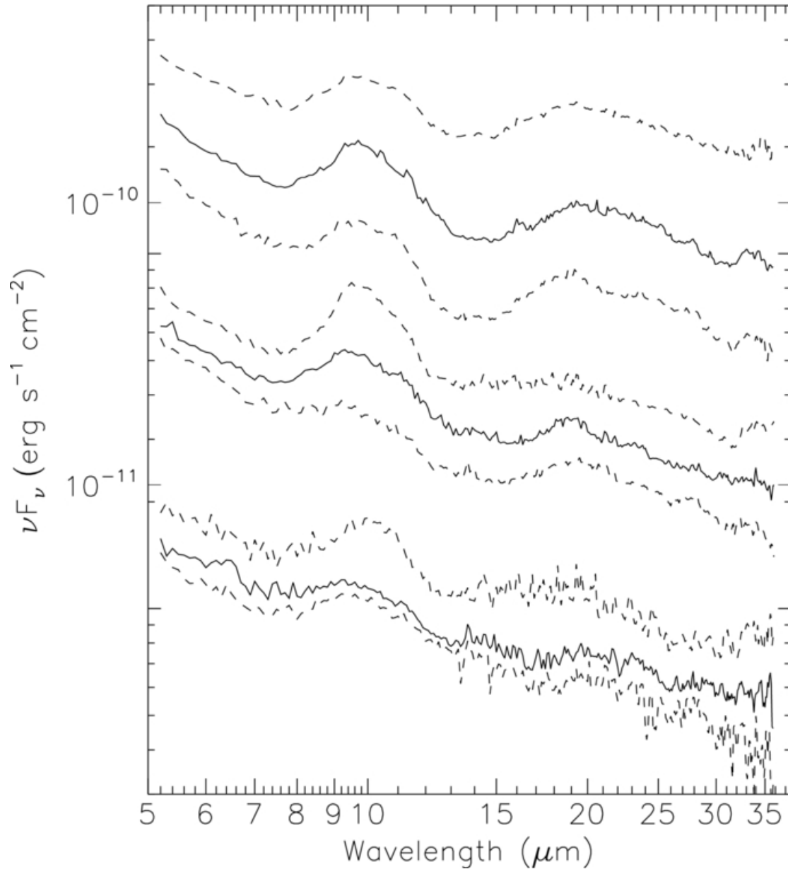
Figure 21. from The Spitzer Infrared Spectrograph Survey of T Tauri Stars in Taurus Furlan et al. 2011 ApJS 195 3 doi:10.1088/0067-0049/195/1/3 https://dx.doi.org/10.1088/0067-0049/195/1/3 © 2011. The American Astronomical Society. All rights reserved.
