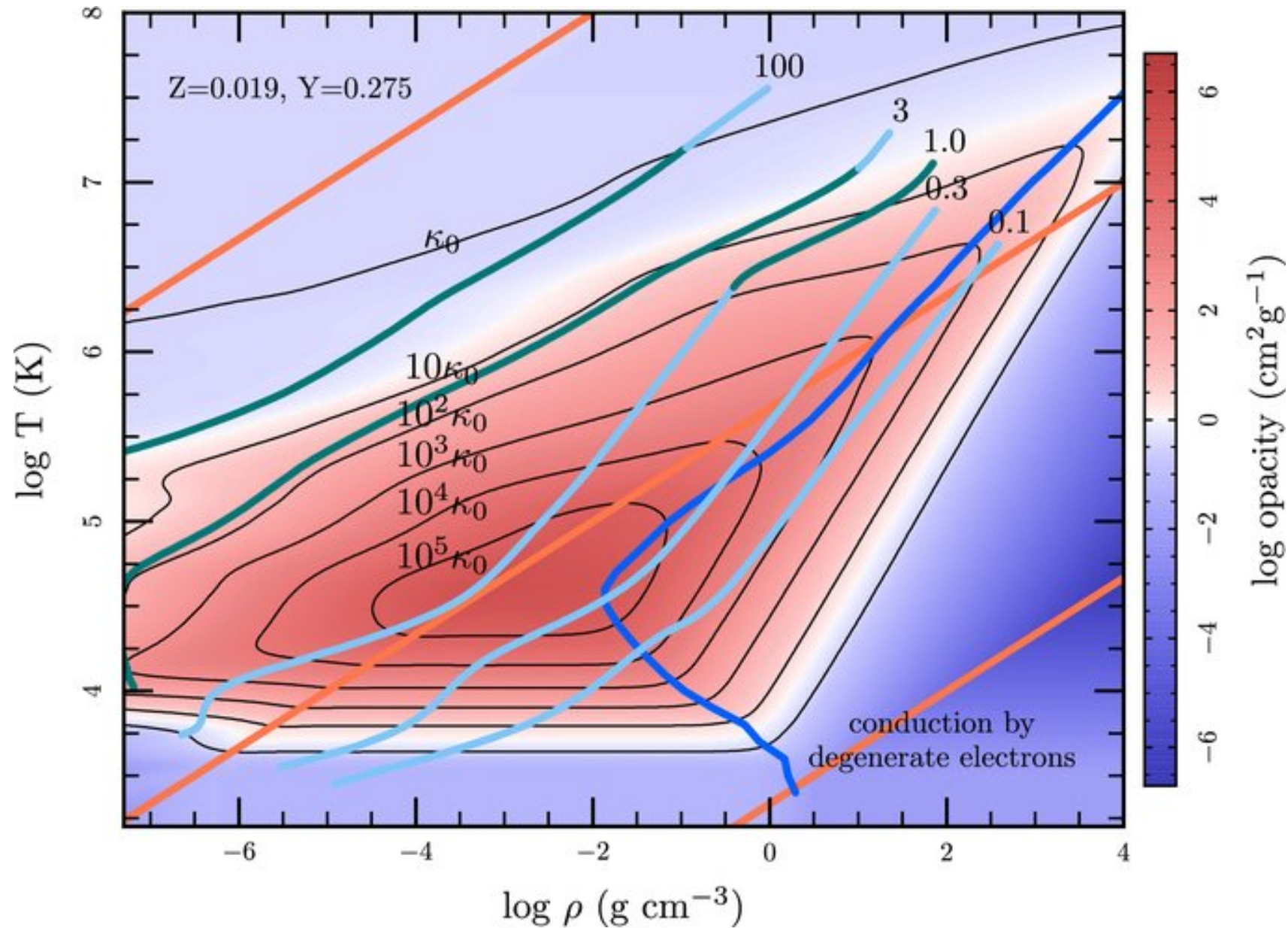
Figure 3. from Modules for Experiments in Stellar Astrophysics (MESA) Paxton et al. 2011 ApJS 192 3 doi:10.1088/0067-0049/192/1/3 https://dx.doi.org/10.1088/0067-0049/192/1/3 © 2011. The American Astronomical Society. All rights reserved.
