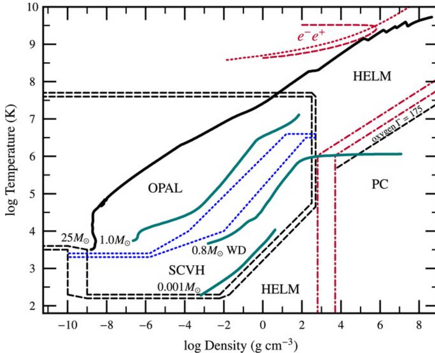
Figure 1. from Modules for Experiments in Stellar Astrophysics (MESA) Paxton et al. 2011 ApJS 192 3 doi:10.1088/0067-0049/192/1/3 https://dx.doi.org/10.1088/0067-0049/192/1/3 © 2011. The American Astronomical Society. All rights reserved.
