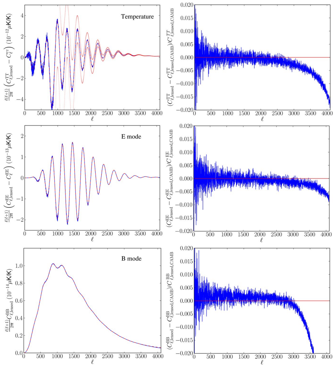
Figure 8. from Fast and Optimal Cosmic Microwave Background Lensing Using Statistical Interpolation on the Sphere LAVAUX & WANDELT 2010 ApJS 191 32 doi:10.1088/0067-0049/191/1/32 https://dx.doi.org/10.1088/0067-0049/191/1/32 © 2010. The American Astronomical Society. All rights reserved.
