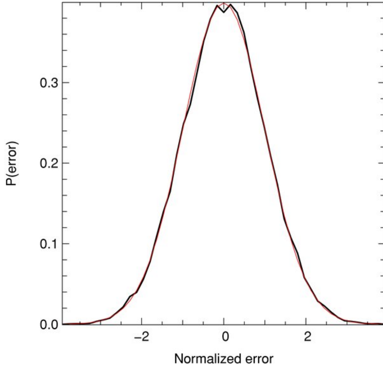
Figure 5. from Fast and Optimal Cosmic Microwave Background Lensing Using Statistical Interpolation on the Sphere LAVAUX & WANDELT 2010 ApJS 191 32 doi:10.1088/0067-0049/191/1/32 https://dx.doi.org/10.1088/0067-0049/191/1/32 © 2010. The American Astronomical Society. All rights reserved.
