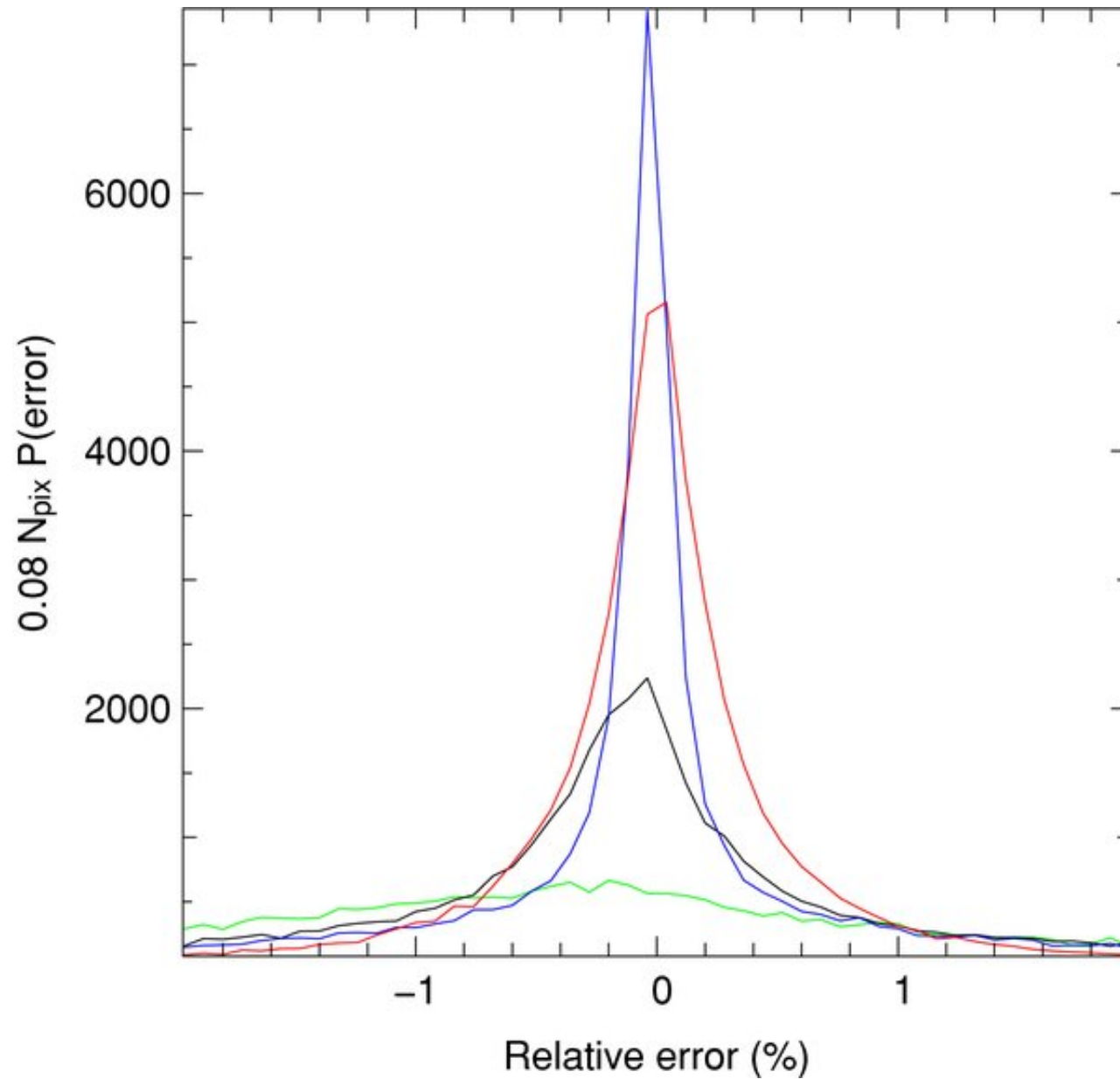
Figure 4. from Fast and Optimal Cosmic Microwave Background Lensing Using Statistical Interpolation on the Sphere LAVAUX & WANDELT 2010 ApJS 191 32 doi:10.1088/0067-0049/191/1/32 https://dx.doi.org/10.1088/0067-0049/191/1/32 © 2010. The American Astronomical Society. All rights reserved.
