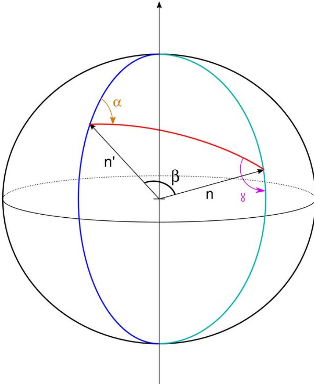
Figure 2. from Fast and Optimal Cosmic Microwave Background Lensing Using Statistical Interpolation on the Sphere LAVAUX & WANDELT 2010 ApJS 191 32 doi:10.1088/0067-0049/191/1/32 https://dx.doi.org/10.1088/0067-0049/191/1/32 © 2010. The American Astronomical Society. All rights reserved.
