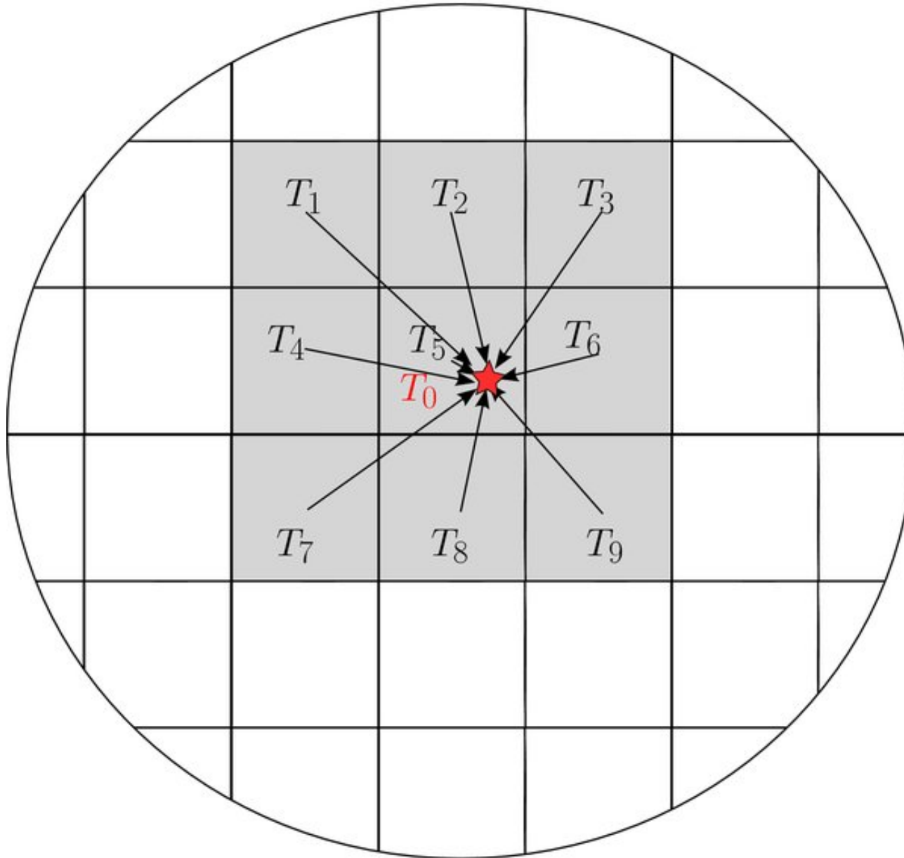
Figure 1. from Fast and Optimal Cosmic Microwave Background Lensing Using Statistical Interpolation on the Sphere LAVAUX & WANDELT 2010 ApJS 191 32 doi:10.1088/0067-0049/191/1/32 https://dx.doi.org/10.1088/0067-0049/191/1/32 © 2010. The American Astronomical Society. All rights reserved.
