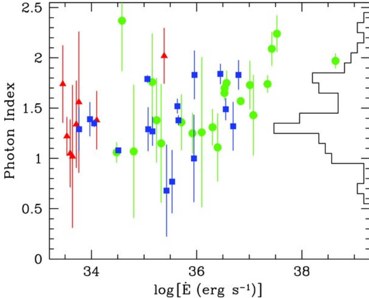
Figure 8. from The First Fermi Large Area Telescope Catalog of Gamma-ray Pulsars ABDO ET AL. 2010 ApJS 187 460 doi:10.1088/0067-0049/187/2/460 https://dx.doi.org/10.1088/0067-0049/187/2/460 © 2010. The American Astronomical Society. All rights reserved.
