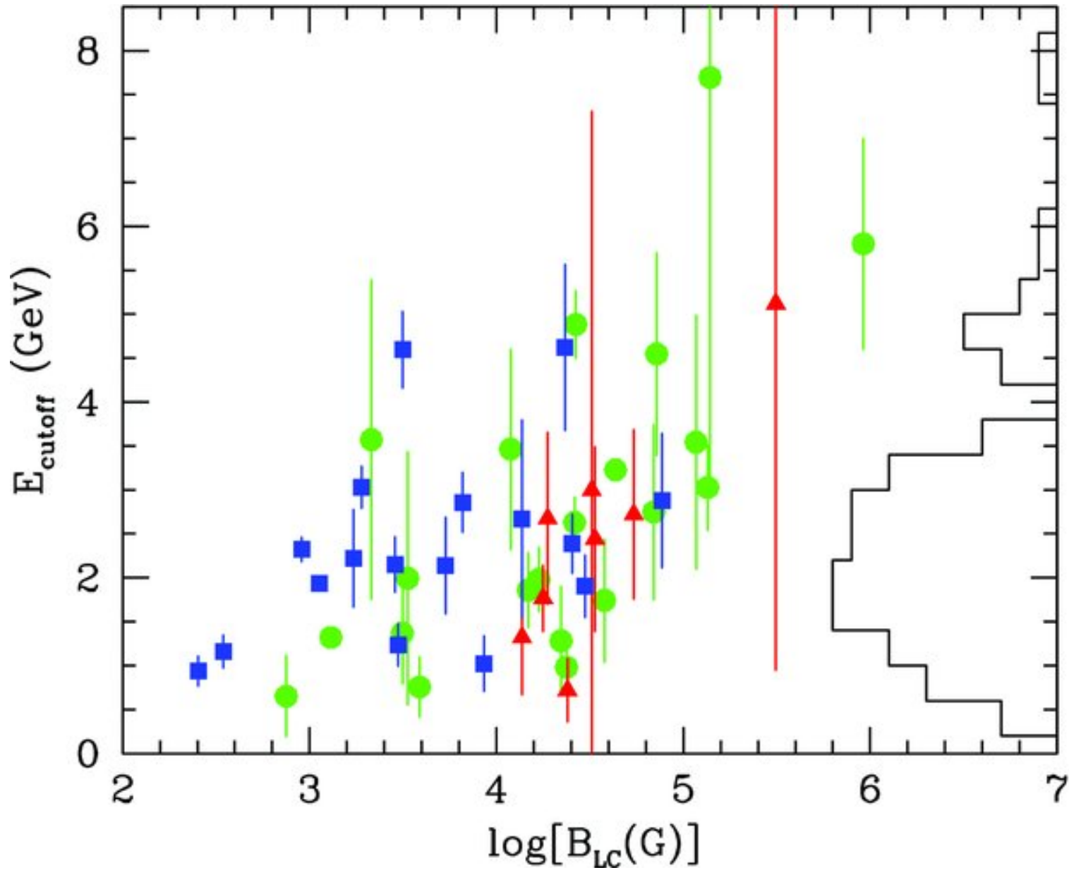
Figure 7. from The First Fermi Large Area Telescope Catalog of Gamma-ray Pulsars ABDO ET AL. 2010 ApJS 187 460 doi:10.1088/0067-0049/187/2/460 https://dx.doi.org/10.1088/0067-0049/187/2/460 © 2010. The American Astronomical Society. All rights reserved.
