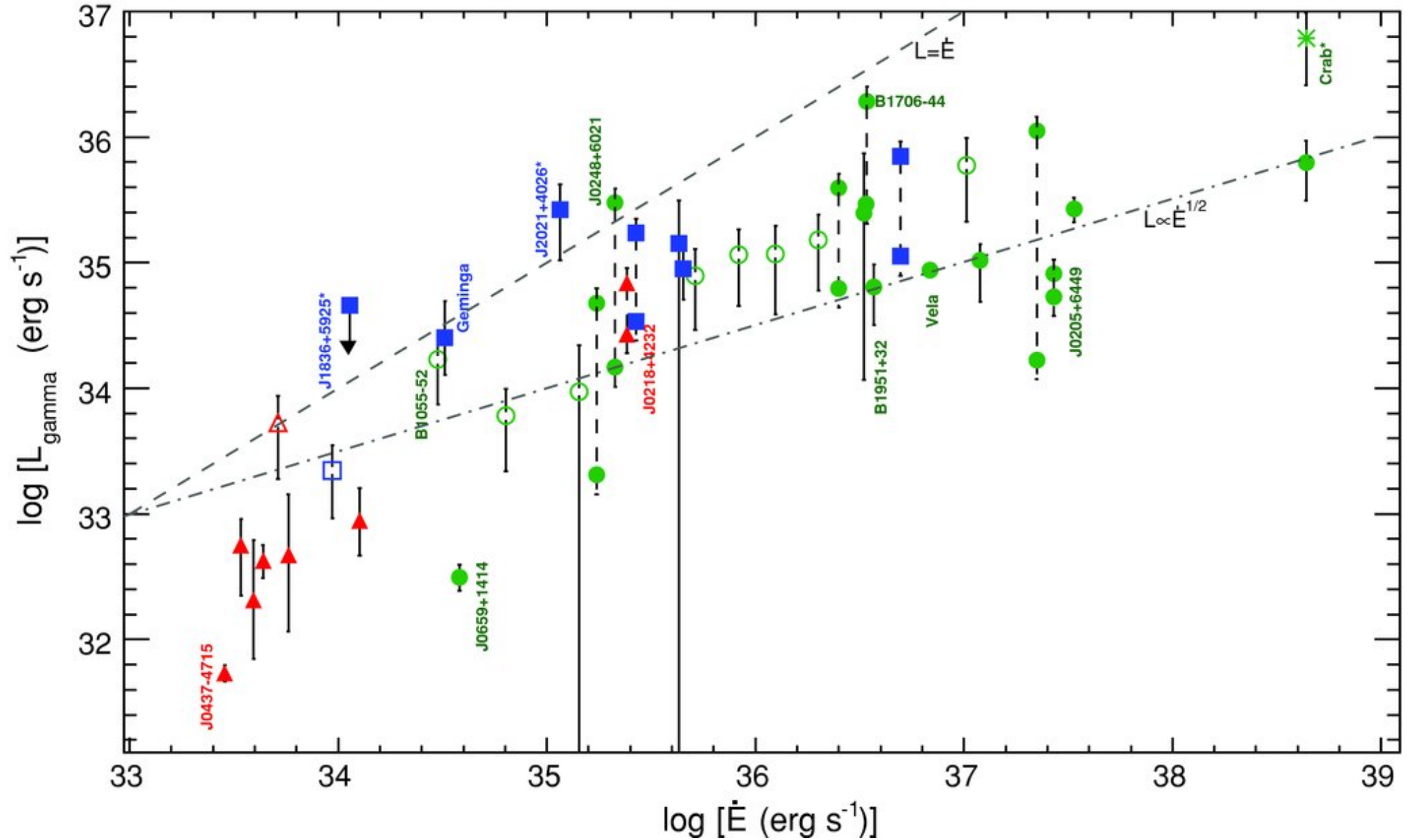
Figure 6. from The First Fermi Large Area Telescope Catalog of Gamma-ray Pulsars ABDO ET AL. 2010 ApJS 187 460 doi:10.1088/0067-0049/187/2/460 https://dx.doi.org/10.1088/0067-0049/187/2/460 © 2010. The American Astronomical Society. All rights reserved.
