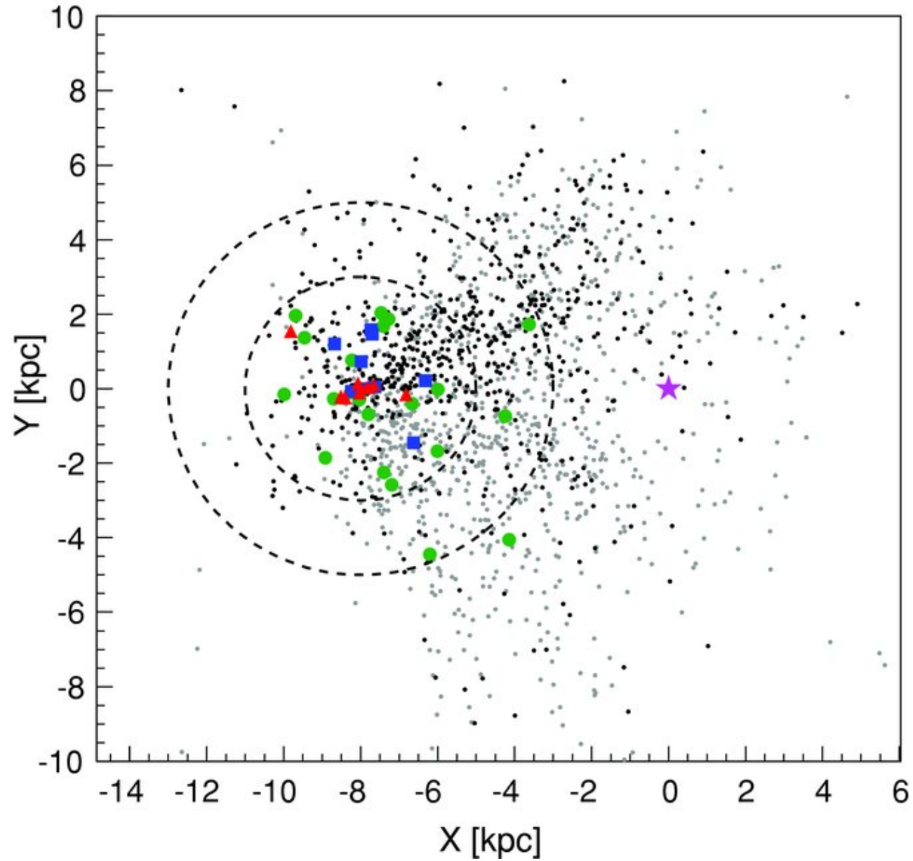
Figure 3. from The First Fermi Large Area Telescope Catalog of Gamma-ray Pulsars ABDO ET AL. 2010 ApJS 187 460 doi:10.1088/0067-0049/187/2/460 https://dx.doi.org/10.1088/0067-0049/187/2/460 © 2010. The American Astronomical Society. All rights reserved.
