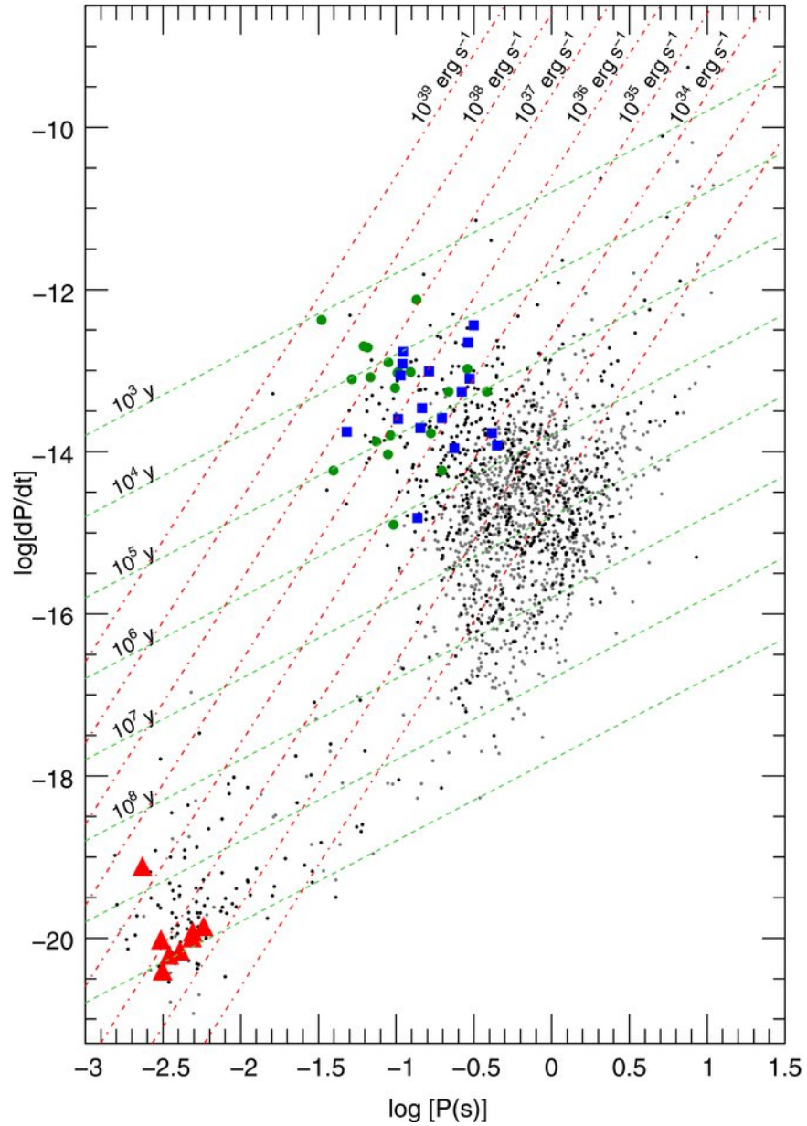
Figure 2. from The First Fermi Large Area Telescope Catalog of Gamma-ray Pulsars ABDO ET AL. 2010 ApJS 187 460 doi:10.1088/0067-0049/187/2/460 https://dx.doi.org/10.1088/0067-0049/187/2/460 © 2010. The American Astronomical Society. All rights reserved.
