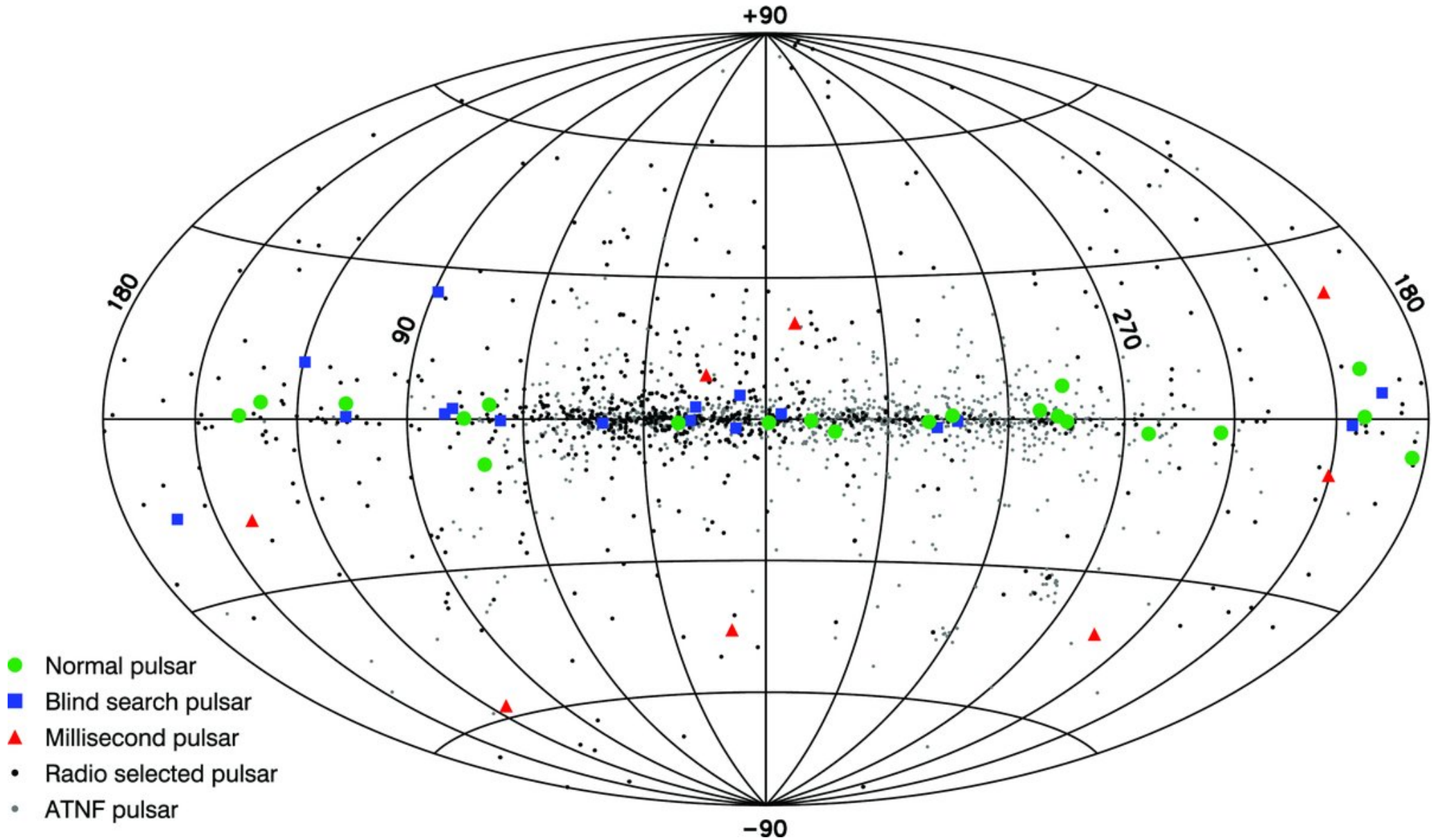
Figure 1. from The First Fermi Large Area Telescope Catalog of Gamma-ray Pulsars ABDO ET AL. 2010 ApJS 187 460 doi:10.1088/0067-0049/187/2/460 https://dx.doi.org/10.1088/0067-0049/187/2/460 © 2010. The American Astronomical Society. All rights reserved.
