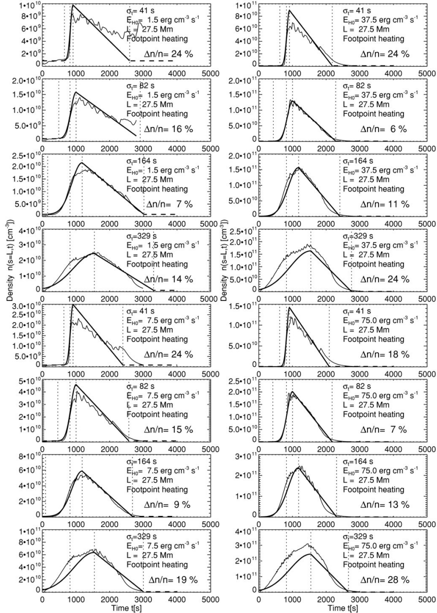
Figure 9. from The Hydrodynamic Evolution of Impulsively Heated Coronal Loops: Explicit Analytical Approximations ASCHWANDEN & TSIKLARI 2009 ApJS 185 171 doi:10.1088/0067-0049/185/1/171 https://dx.doi.org/10.1088/0067-0049/185/1/171
