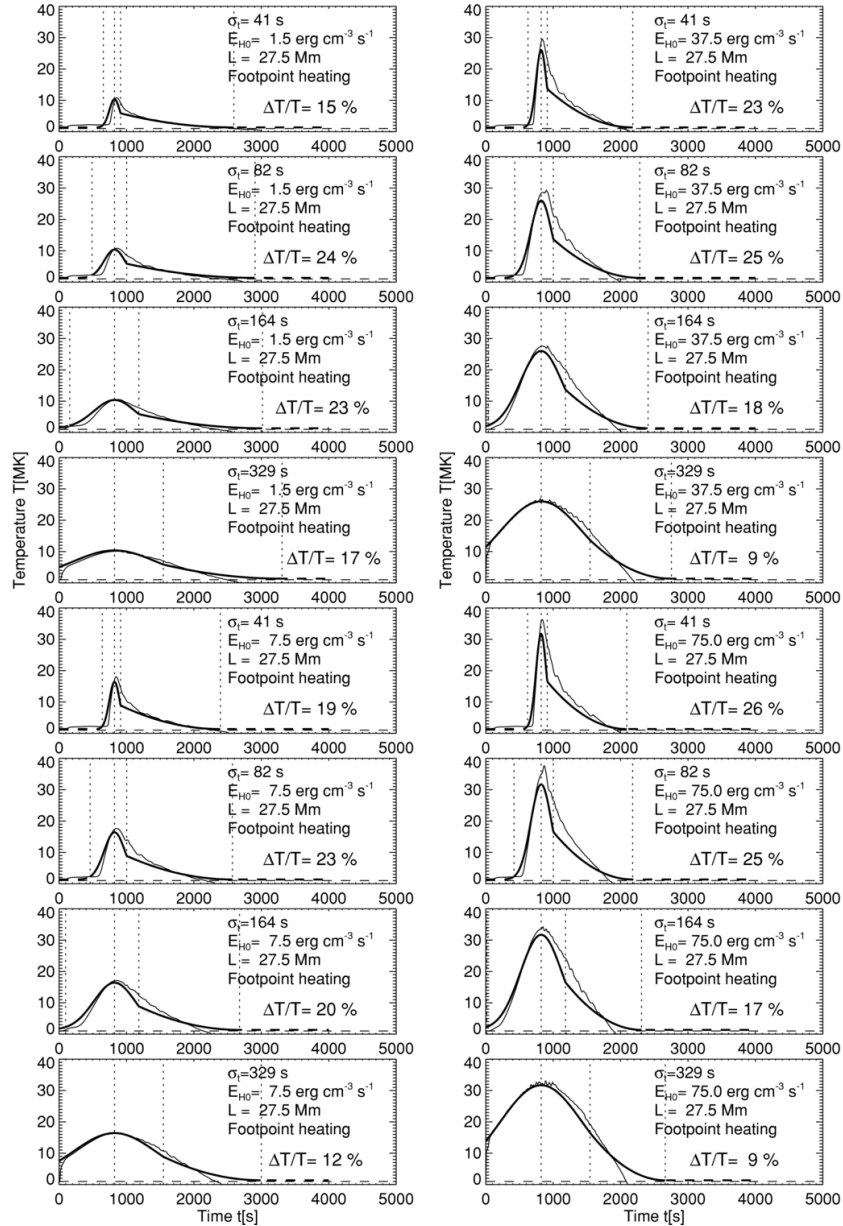
Figure 8. from The Hydrodynamic Evolution of Impulsively Heated Coronal Loops: Explicit Analytical Approximations ASCHWANDEN & TSIKLARI 2009 ApJS 185 171 doi:10.1088/0067-0049/185/1/171 https://dx.doi.org/10.1088/0067-0049/185/1/171
