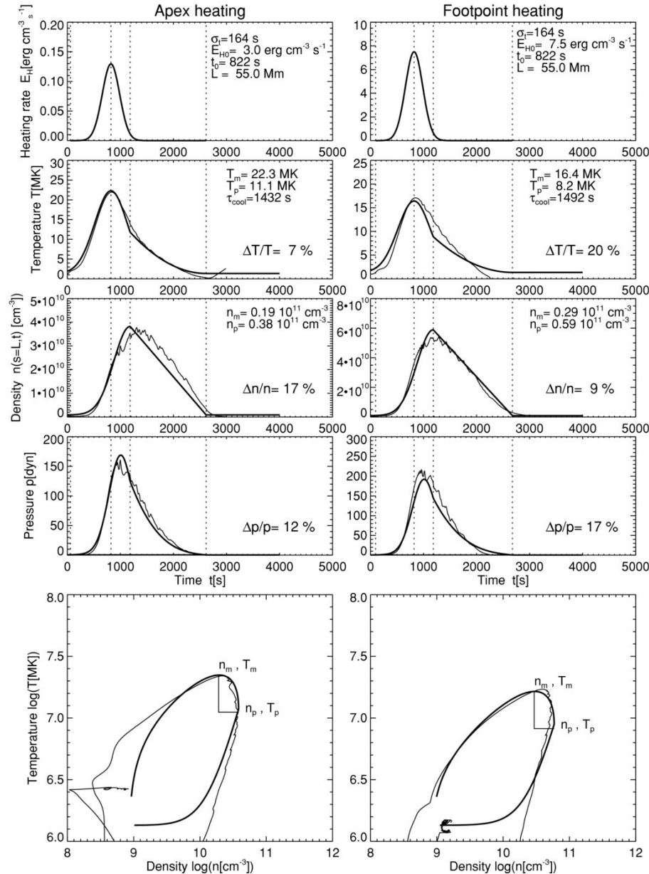
Figure 7. from The Hydrodynamic Evolution of Impulsively Heated Coronal Loops: Explicit Analytical Approximations ASCHWANDEN & TSIKLARI 2009 ApJS 185 171 doi:10.1088/0067-0049/185/1/171 https://dx.doi.org/10.1088/0067-0049/185/1/171
