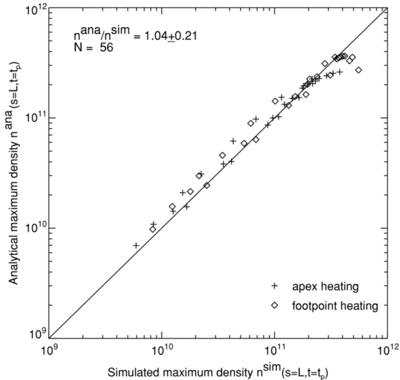
Figure 6. from The Hydrodynamic Evolution of Impulsively Heated Coronal Loops: Explicit Analytical Approximations ASCHWANDEN & TSIKLARI 2009 ApJS 185 171 doi:10.1088/0067-0049/185/1/171 https://dx.doi.org/10.1088/0067-0049/185/1/171 © 2009. The American Astronomical Society. All rights reserved.
