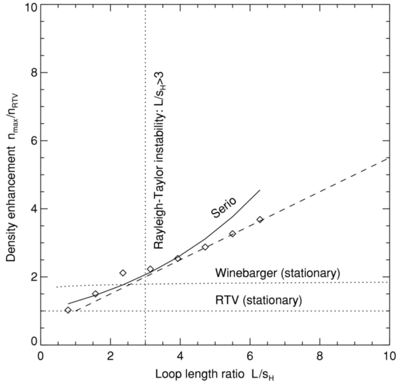
Figure 5. from The Hydrodynamic Evolution of Impulsively Heated Coronal Loops: Explicit Analytical Approximations ASCHWANDEN & TSIKLARI 2009 ApJS 185 171 doi:10.1088/0067-0049/185/1/171 https://dx.doi.org/10.1088/0067-0049/185/1/171 © 2009. The American Astronomical Society. All rights reserved.
