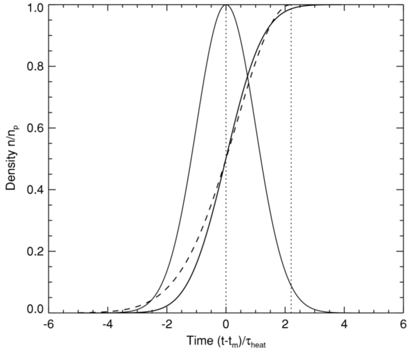
Figure 4. from The Hydrodynamic Evolution of Impulsively Heated Coronal Loops: Explicit Analytical Approximations ASCHWANDEN & TSIKLARI 2009 ApJS 185 171 doi:10.1088/0067-0049/185/1/171 https://dx.doi.org/10.1088/0067-0049/185/1/171 © 2009. The American Astronomical Society. All rights reserved.
