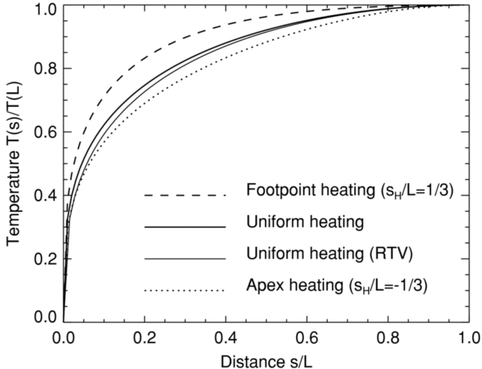
Figure 2. from The Hydrodynamic Evolution of Impulsively Heated Coronal Loops: Explicit Analytical Approximations ASCHWANDEN & TSIKLARI 2009 ApJS 185 171 doi:10.1088/0067-0049/185/1/171 https://dx.doi.org/10.1088/0067-0049/185/1/171 © 2009. The American Astronomical Society. All rights reserved.
