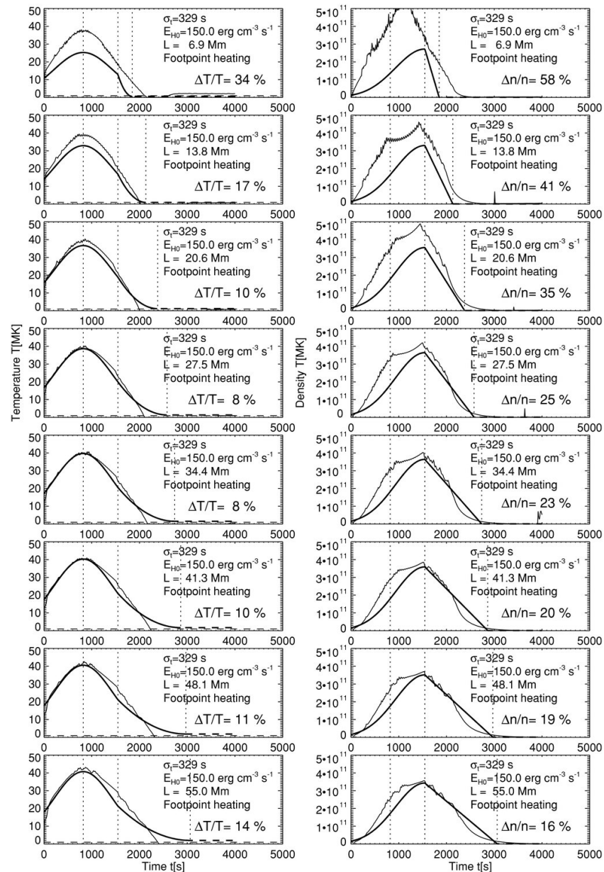
Figure 10. from The Hydrodynamic Evolution of Impulsively Heated Coronal Loops: Explicit Analytical Approximations ASCHWANDEN & TSIKLARI 2009 ApJS 185 171 doi:10.1088/0067-0049/185/1/171 https://dx.doi.org/10.1088/0067-0049/185/1/171
