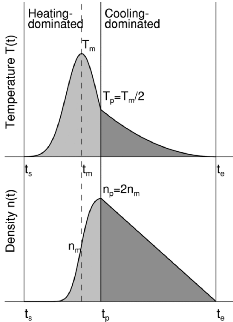
Figure 1. from The Hydrodynamic Evolution of Impulsively Heated Coronal Loops: Explicit Analytical Approximations ASCHWANDEN & TSIKLARI 2009 ApJS 185 171 doi:10.1088/0067-0049/185/1/171 https://dx.doi.org/10.1088/0067-0049/185/1/171 © 2009. The American Astronomical Society. All rights reserved.
