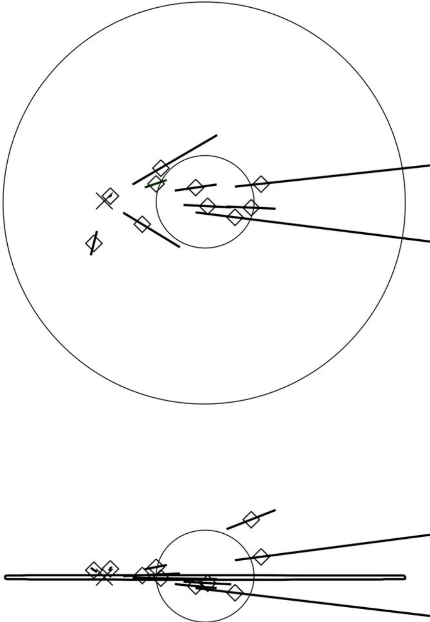
Figure 69. from Comprehensive Photometric Histories of All Known Galactic Recurrent Novae SCHAEFER 2010 ApJS 187 275 doi:10.1088/0067-0049/187/2/275 https://dx.doi.org/10.1088/0067-0049/187/2/275 © 2010. The American Astronomical Society. All rights reserved.
