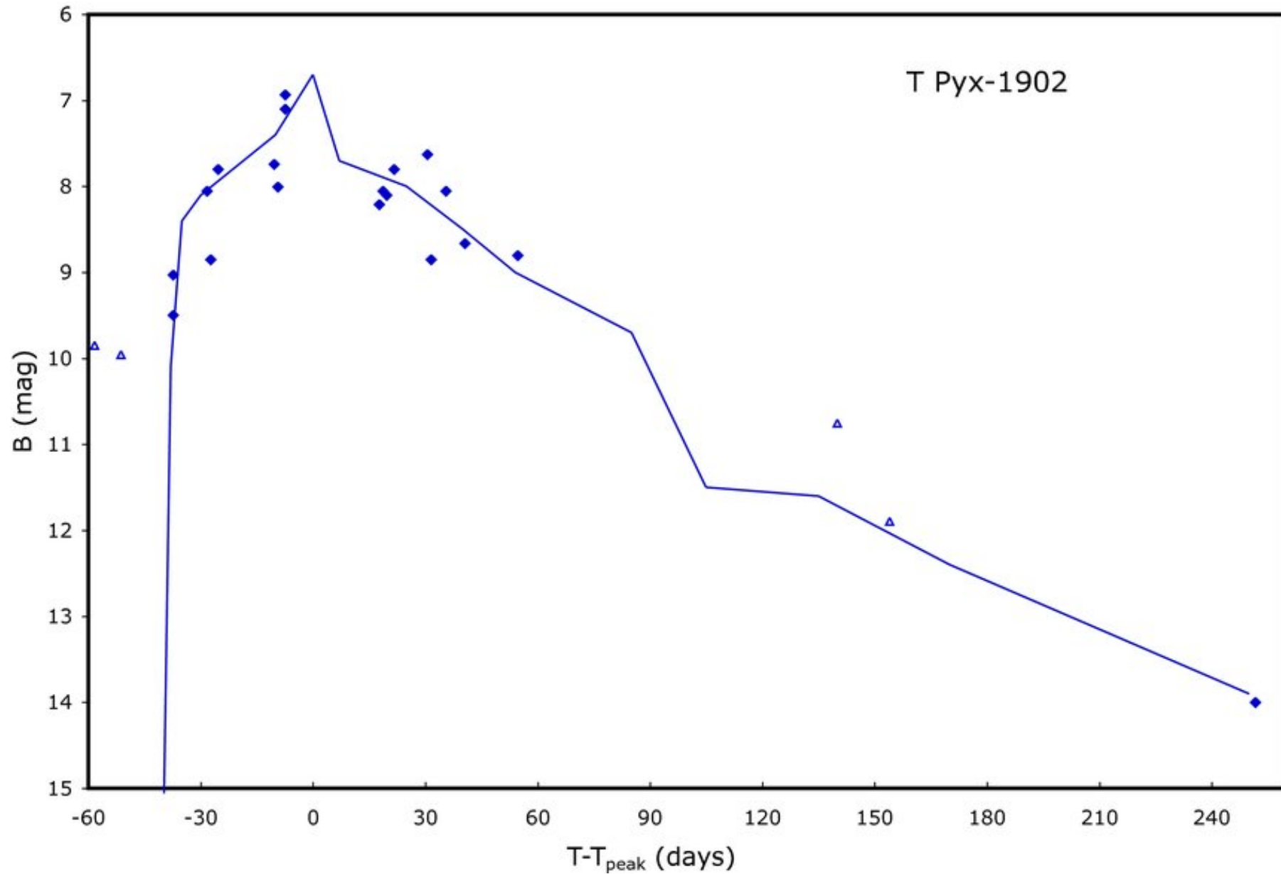
Figure 2. from Comprehensive Photometric Histories of All Known Galactic Recurrent Novae SCHAEFER 2010 ApJS 187 275 doi:10.1088/0067-0049/187/2/275 https://dx.doi.org/10.1088/0067-0049/187/2/275 © 2010. The American Astronomical Society. All rights reserved.
