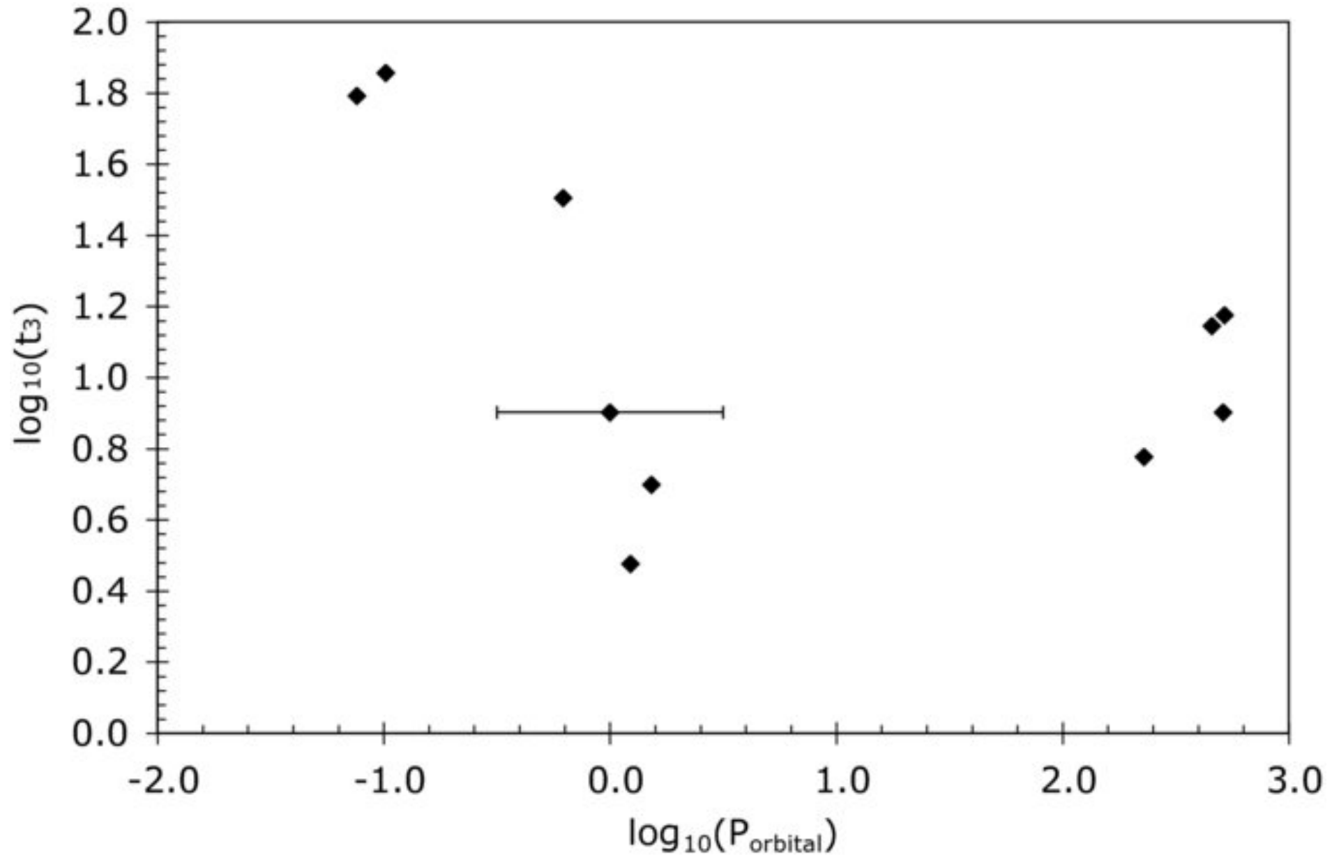
Figure 1. from Comprehensive Photometric Histories of All Known Galactic Recurrent Novae SCHAEFER 2010 ApJS 187 275 doi:10.1088/0067-0049/187/2/275 https://dx.doi.org/10.1088/0067-0049/187/2/275 © 2010. The American Astronomical Society. All rights reserved.
