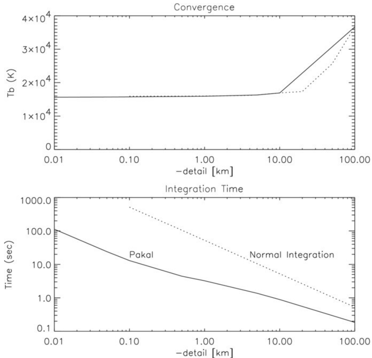
Figure 9. from Pakal: A Three-dimensional Model to Solve the Radiative Transfer Equation DE LA LUZ ET AL. 2010 ApJS 188 437 doi:10.1088/0067-0049/188/2/437 https://dx.doi.org/10.1088/0067-0049/188/2/437 © 2010. The American Astronomical Society. All rights reserved.
