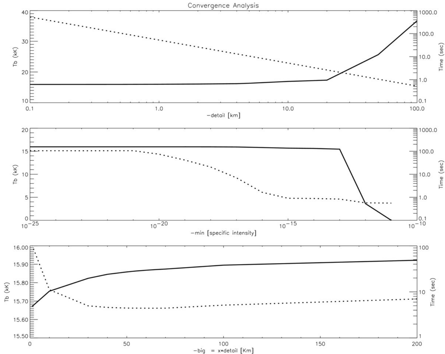
Figure 8. from Pakal: A Three-dimensional Model to Solve the Radiative Transfer Equation DE LA LUZ ET AL. 2010 ApJS 188 437 doi:10.1088/0067-0049/188/2/437 https://dx.doi.org/10.1088/0067-0049/188/2/437 © 2010. The American Astronomical Society. All rights reserved.
