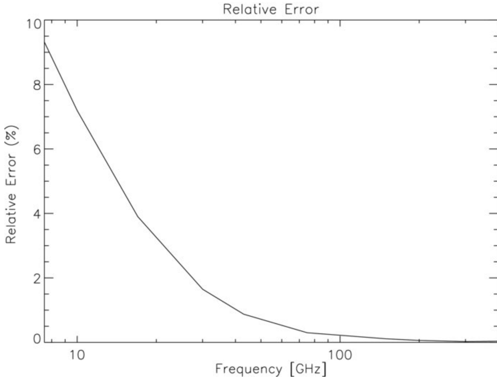
Figure 4. from Pakal: A Three-dimensional Model to Solve the Radiative Transfer Equation DE LA LUZ ET AL. 2010 ApJS 188 437 doi:10.1088/0067-0049/188/2/437 https://dx.doi.org/10.1088/0067-0049/188/2/437 © 2010. The American Astronomical Society. All rights reserved.
