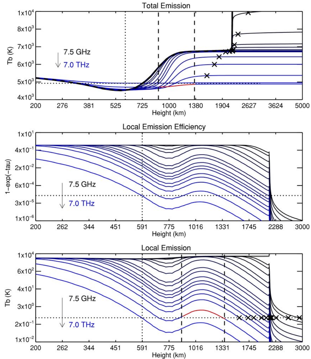
Figure 3. from Pakal: A Three-dimensional Model to Solve the Radiative Transfer Equation DE LA LUZ ET AL. 2010 ApJS 188 437 doi:10.1088/0067-0049/188/2/437 https://dx.doi.org/10.1088/0067-0049/188/2/437 © 2010. The American Astronomical Society. All rights reserved.
