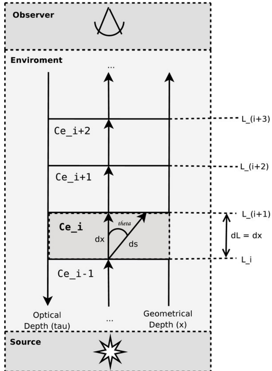
Figure 1. from Pakal: A Three-dimensional Model to Solve the Radiative Transfer Equation DE LA LUZ ET AL. 2010 ApJS 188 437 doi:10.1088/0067-0049/188/2/437 https://dx.doi.org/10.1088/0067-0049/188/2/437 © 2010. The American Astronomical Society. All rights reserved.
