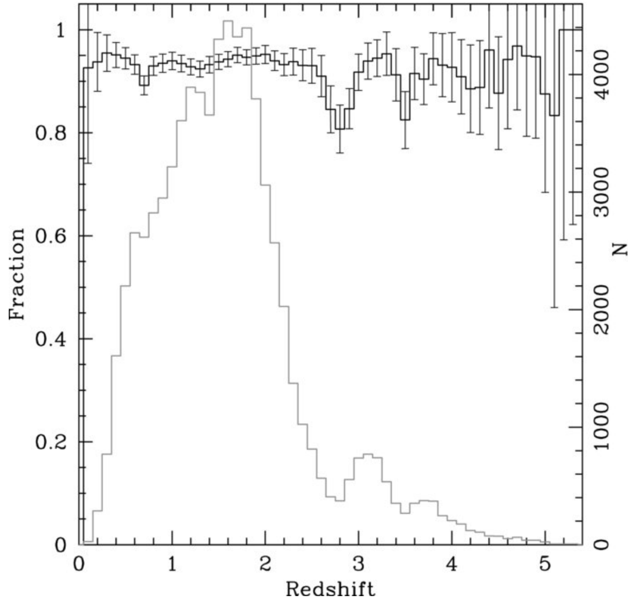
Figure 9. from Efficient Photometric Selection of Quasars from the Sloan Digital Sky Survey. II. 1,000,000 Quasars from Data Release 6 RICHARDS ET AL. 2009 ApJS 180 67 doi:10.1088/0067-0049/180/1/67 https://dx.doi.org/10.1088/0067-0049/180/1/67 © 2009. The American Astronomical Society. All rights reserved.
