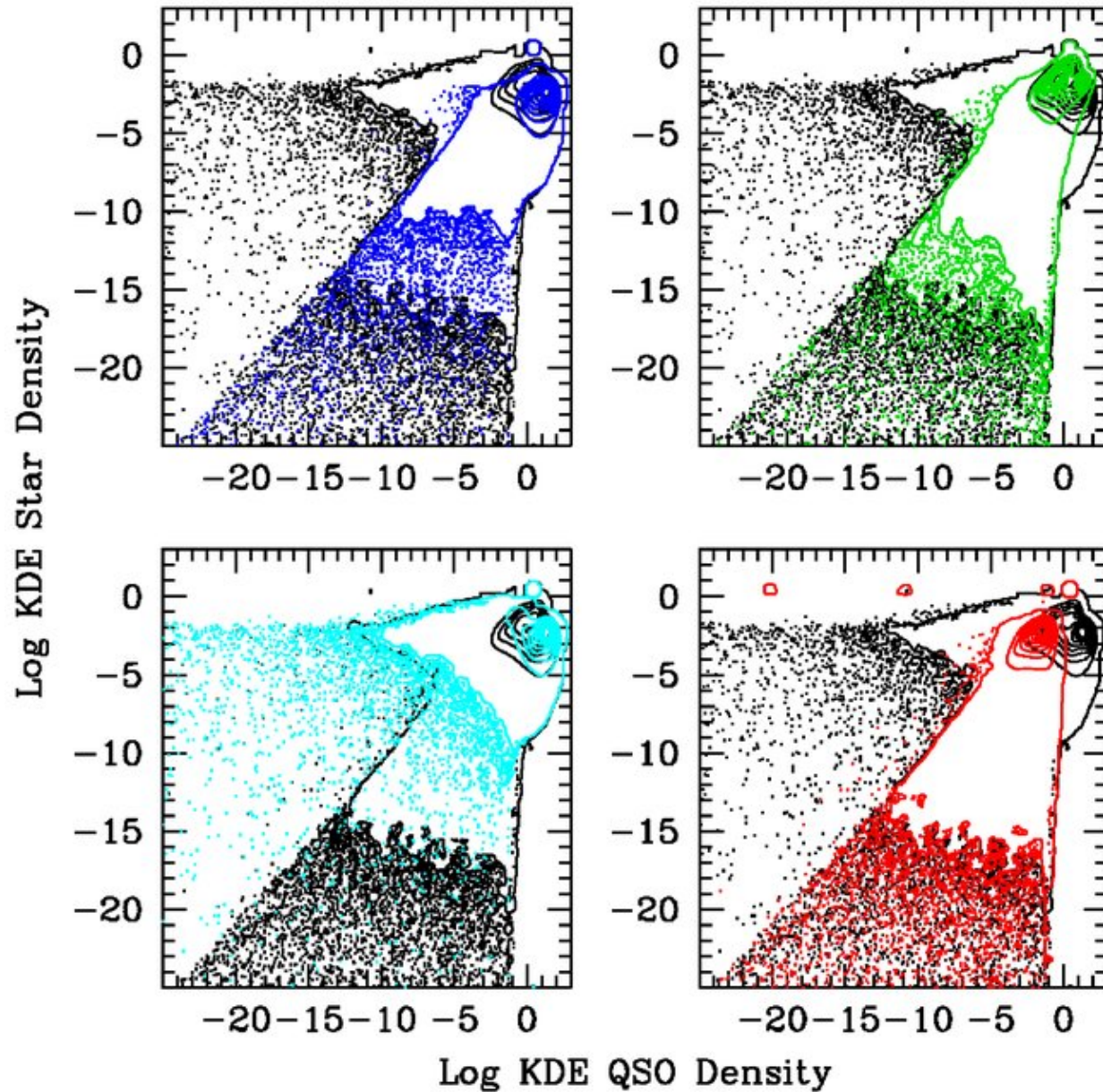
Figure 8. from Efficient Photometric Selection of Quasars from the Sloan Digital Sky Survey. II. 1,000,000 Quasars from Data Release 6 RICHARDS ET AL. 2009 ApJS 180 67 doi:10.1088/0067-0049/180/1/67 https://dx.doi.org/10.1088/0067-0049/180/1/67 © 2009. The American Astronomical Society. All rights reserved.
