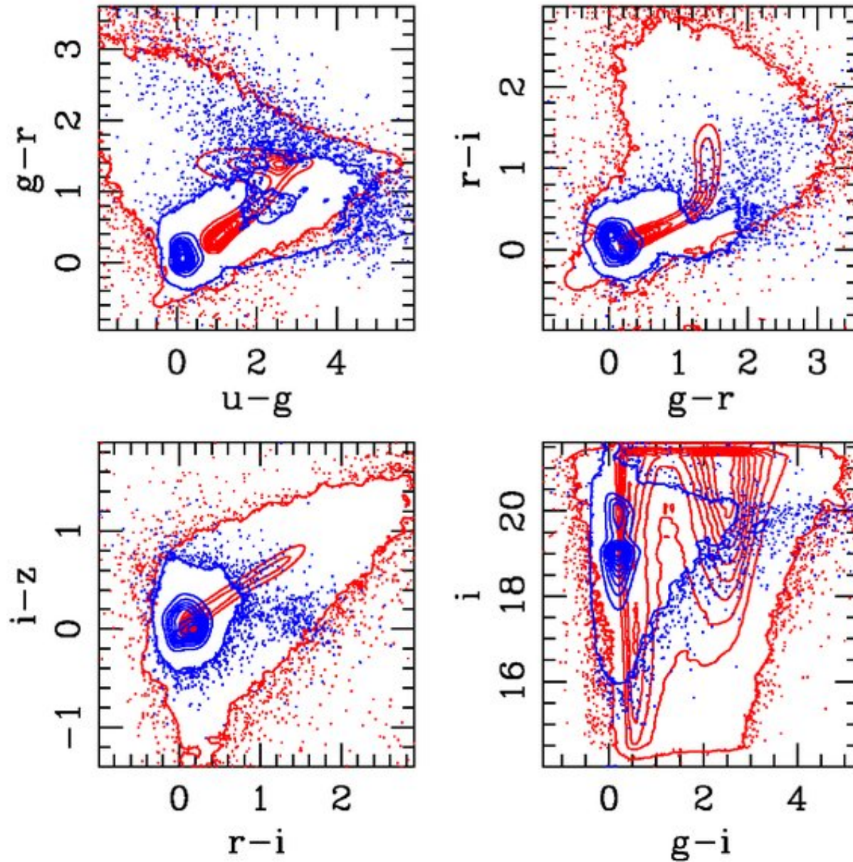
Figure 6. from Efficient Photometric Selection of Quasars from the Sloan Digital Sky Survey. II. 1,000,000 Quasars from Data Release 6 RICHARDS ET AL. 2009 ApJS 180 67 doi:10.1088/0067-0049/180/1/67 https://dx.doi.org/10.1088/0067-0049/180/1/67 © 2009. The American Astronomical Society. All rights reserved.
