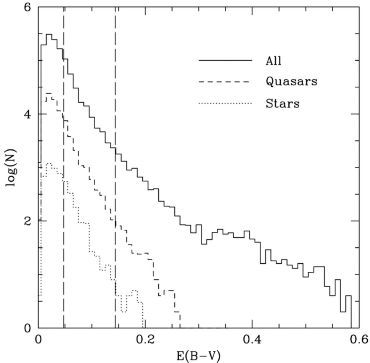
Figure 5. from Efficient Photometric Selection of Quasars from the Sloan Digital Sky Survey. II. 1,000,000 Quasars from Data Release 6 RICHARDS ET AL. 2009 ApJS 180 67 doi:10.1088/0067-0049/180/1/67 https://dx.doi.org/10.1088/0067-0049/180/1/67 © 2009. The American Astronomical Society. All rights reserved.
