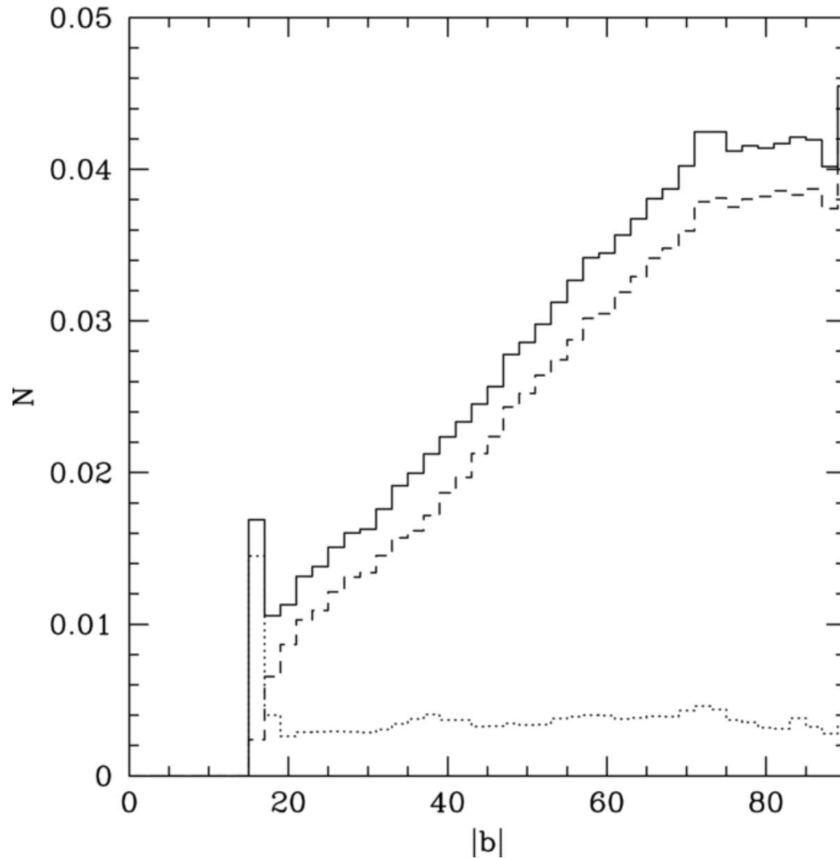
Figure 4. from Efficient Photometric Selection of Quasars from the Sloan Digital Sky Survey. II. 1,000,000 Quasars from Data Release 6 RICHARDS ET AL. 2009 ApJS 180 67 doi:10.1088/0067-0049/180/1/67 https://dx.doi.org/10.1088/0067-0049/180/1/67 © 2009. The American Astronomical Society. All rights reserved.
