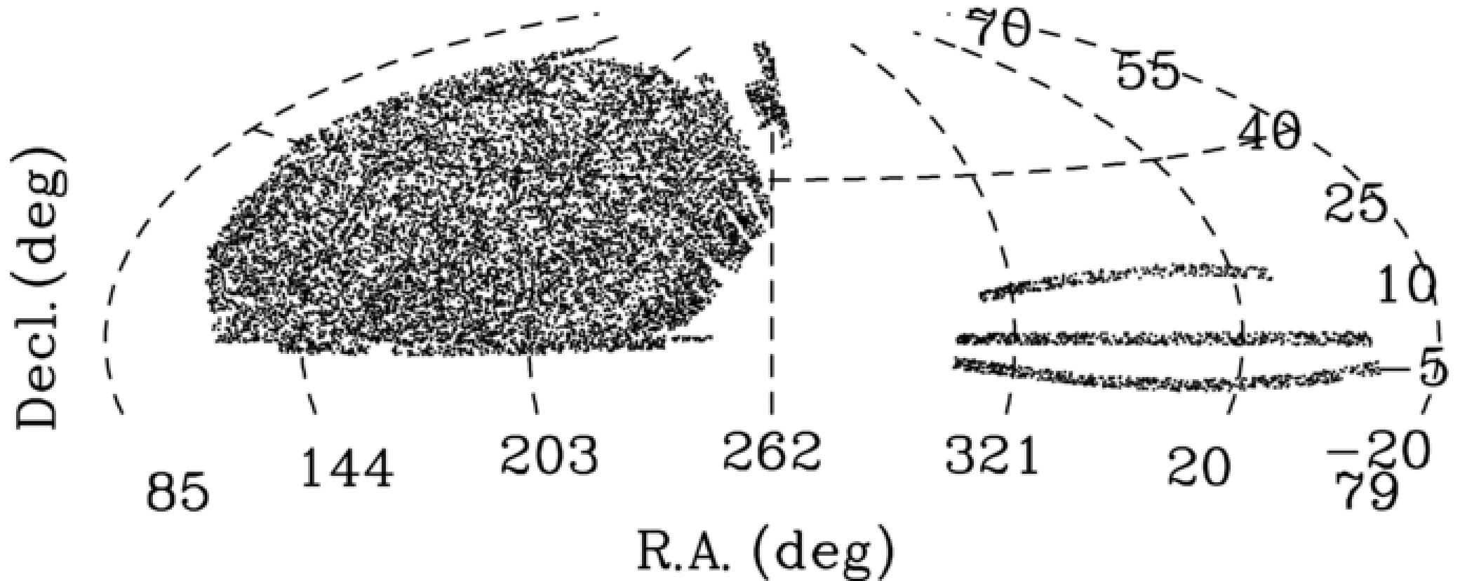
Figure 3. from Efficient Photometric Selection of Quasars from the Sloan Digital Sky Survey. II. 1,000,000 Quasars from Data Release 6 RICHARDS ET AL. 2009 ApJS 180 67 doi:10.1088/0067-0049/180/1/67 https://dx.doi.org/10.1088/0067-0049/180/1/67 © 2009. The American Astronomical Society. All rights reserved.
