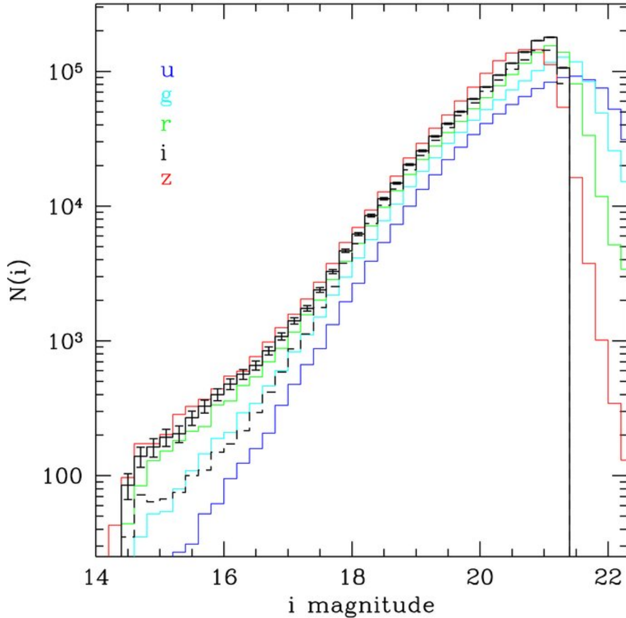
Figure 2. from Efficient Photometric Selection of Quasars from the Sloan Digital Sky Survey. II. 1,000,000 Quasars from Data Release 6 RICHARDS ET AL. 2009 ApJS 180 67 doi:10.1088/0067-0049/180/1/67 https://dx.doi.org/10.1088/0067-0049/180/1/67 © 2009. The American Astronomical Society. All rights reserved.
