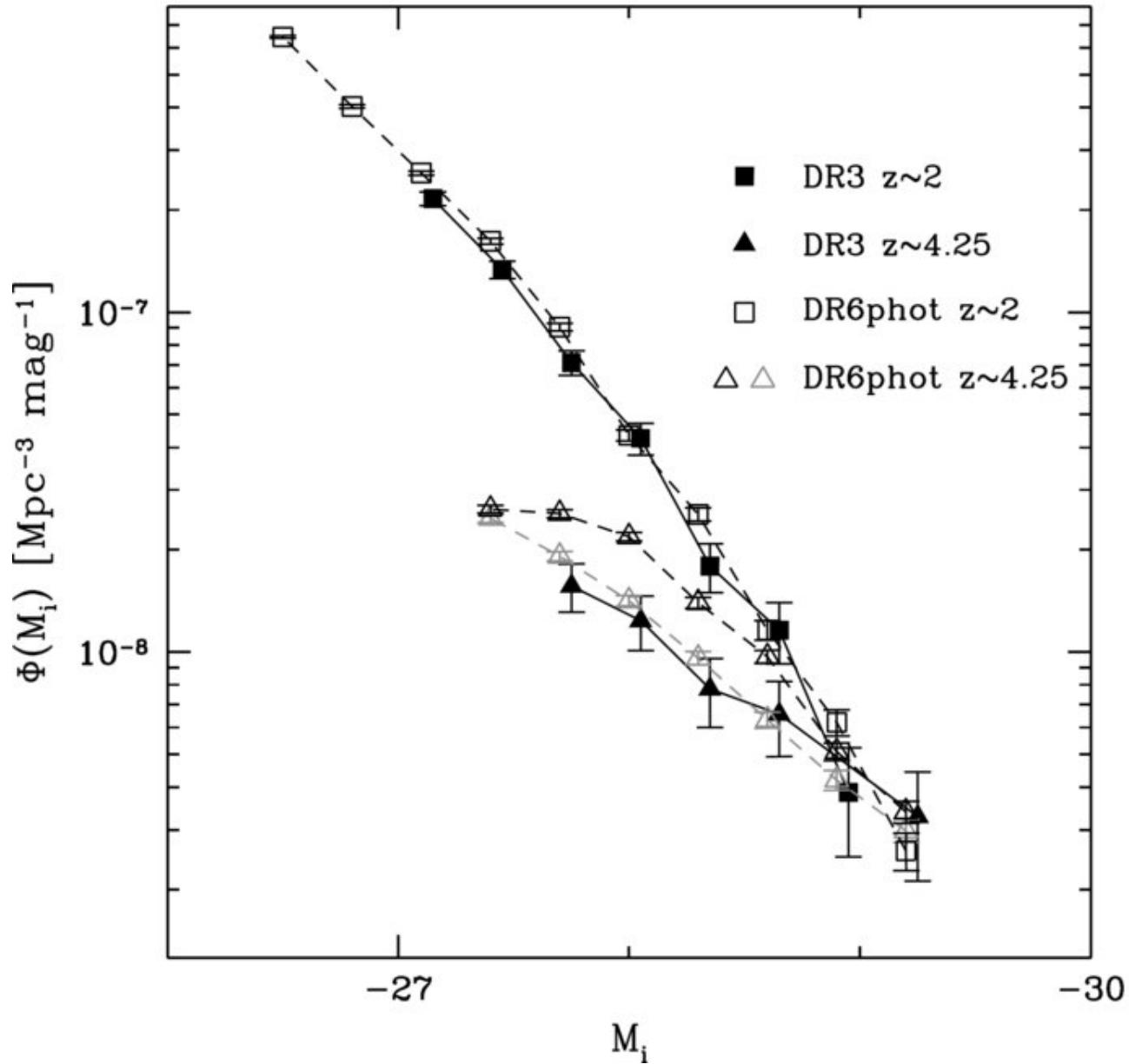
Figure 19. from Efficient Photometric Selection of Quasars from the Sloan Digital Sky Survey. II. 1,000,000 Quasars from Data Release 6 RICHARDS ET AL. 2009 ApJS 180 67 doi:10.1088/0067-0049/180/1/67 https://dx.doi.org/10.1088/0067-0049/180/1/67 © 2009. The American Astronomical Society. All rights reserved.
